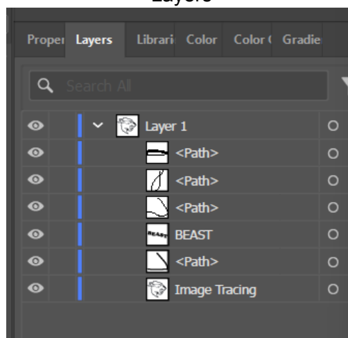
Layers
